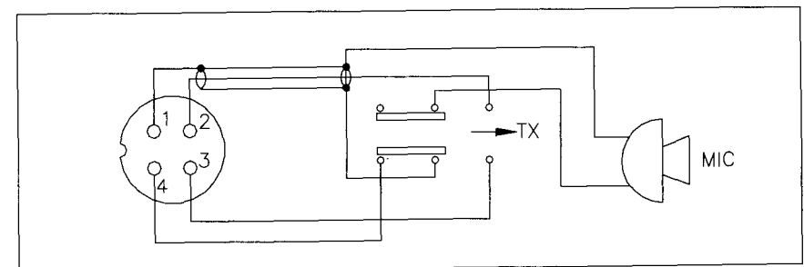
Fig. 1 Schematic of microphone
