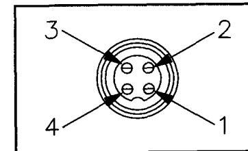
Fig 3. Microphone pin numbers.
